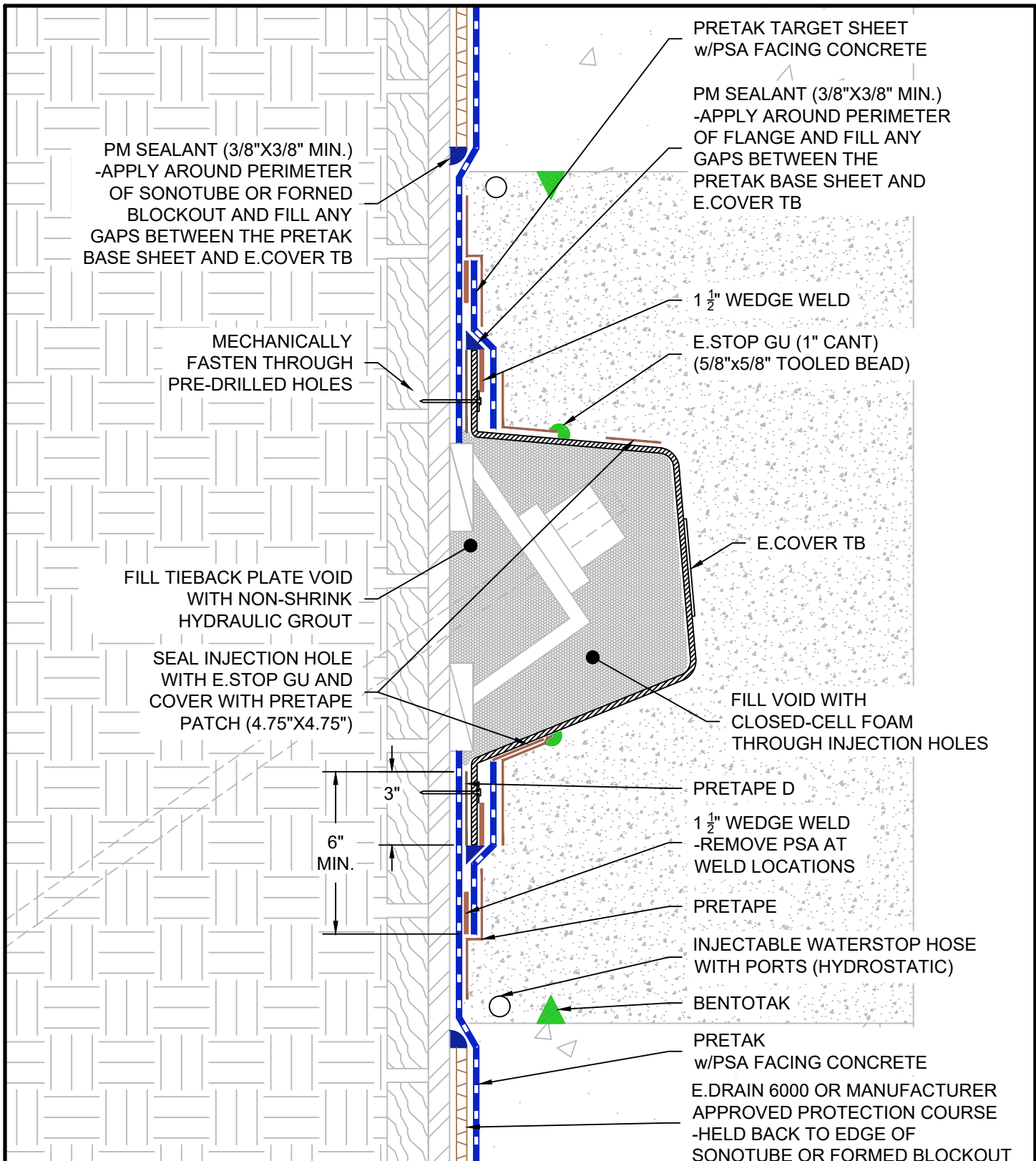
BLINDSIDE VERTICAL TIEBACK - DETENSIONED - E. COVER TB - 28" MIN. SONOTUBE OR FRAMED BLOCKOUT (MIN. 18") - DETAIL
