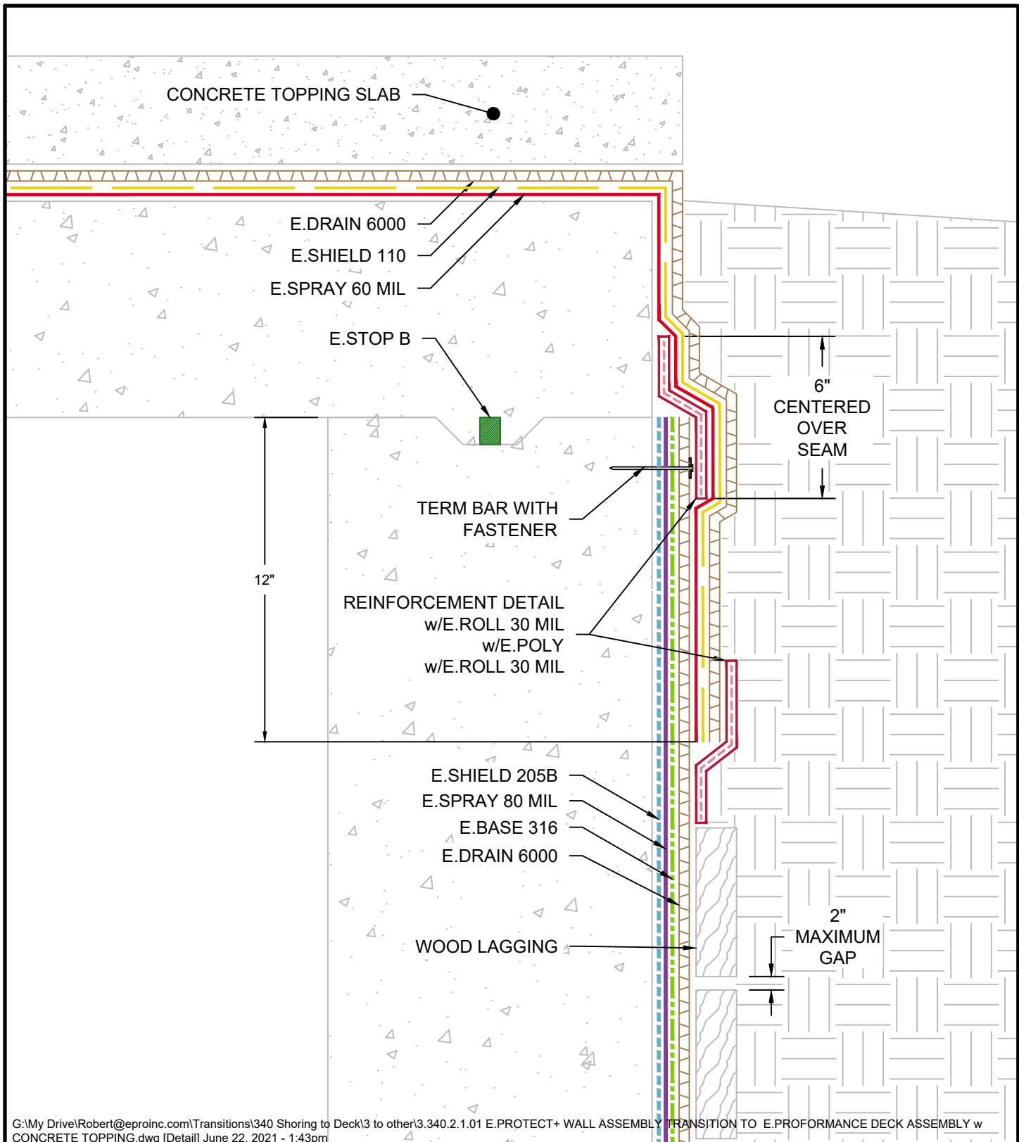
E.PROTECT+ SHORING WALL ASSEMBLY - WOOD LAGGING - TRANSITION TO E.PROFORMANCE DECK ASSEMBLY w/CONCRETE TOPPING
