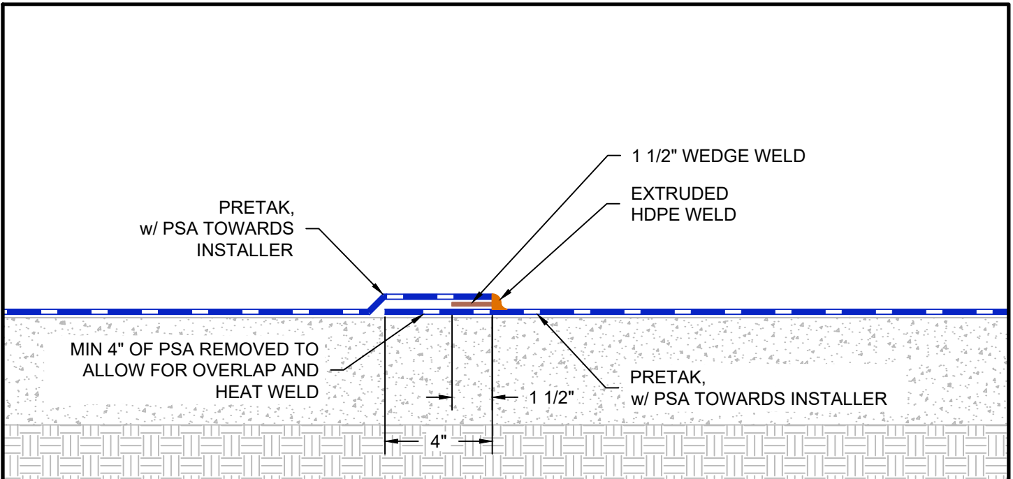
Ⓒ EXTRUDED HEAT WELD w/ WEDGE WELD
