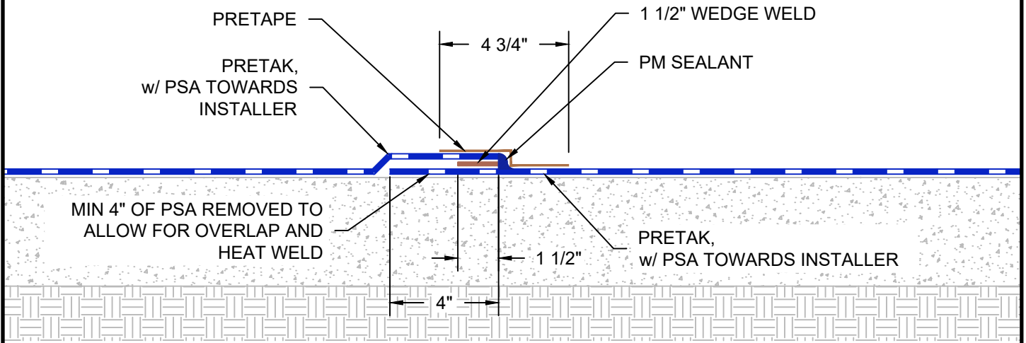
Ⓓ DETAIL WELD w/ WEDGE WELD
