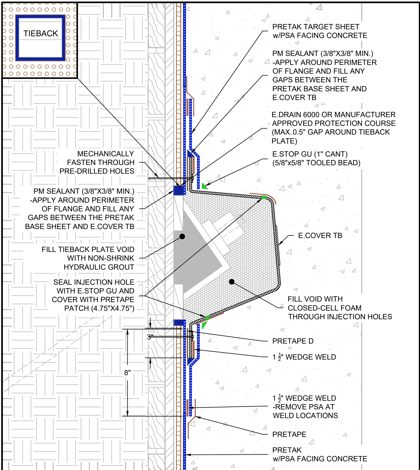
BLINDSIDE VERTICAL TIEBACK - NON-DETENSIONED - E.COVER TB
