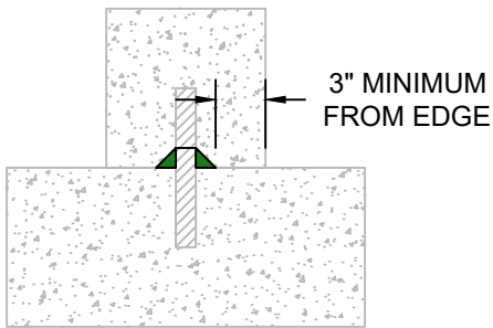
SECTION "A" FRONT VIEW
